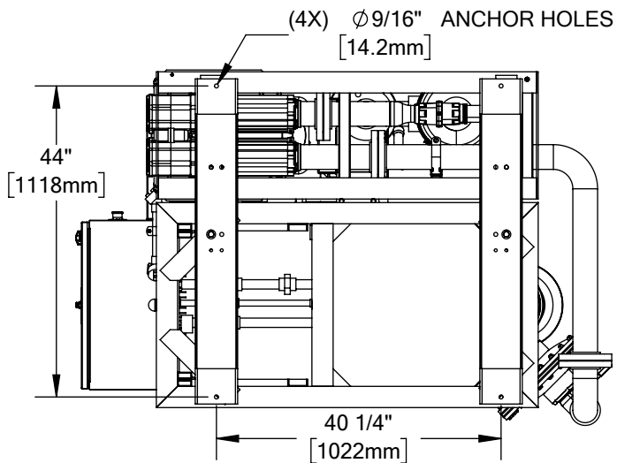
VIEW FROM BOTTOM OF UNIT
