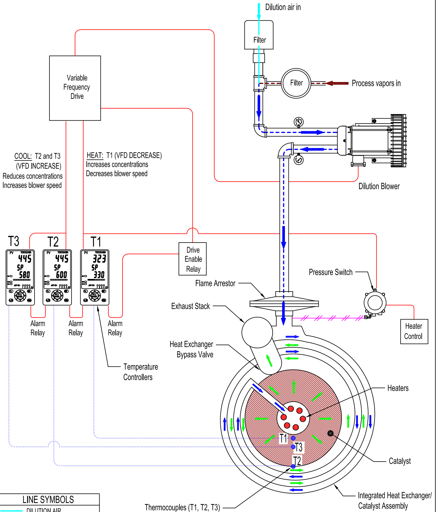
FIGURE 3B: FALCO 600 VFD FLOW AND CONTROL
