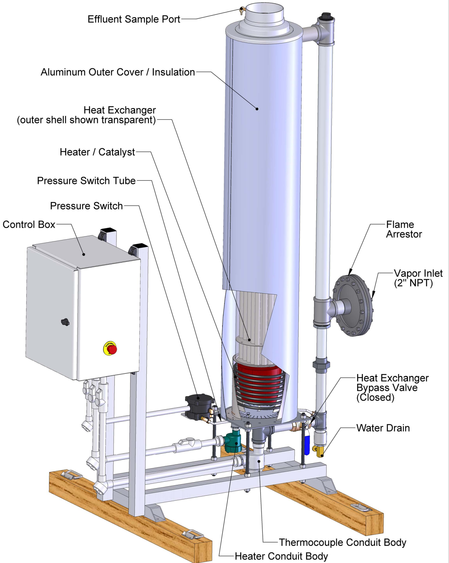
FIGURE 1: FALCO 100 MAJOR COMPONENTS
