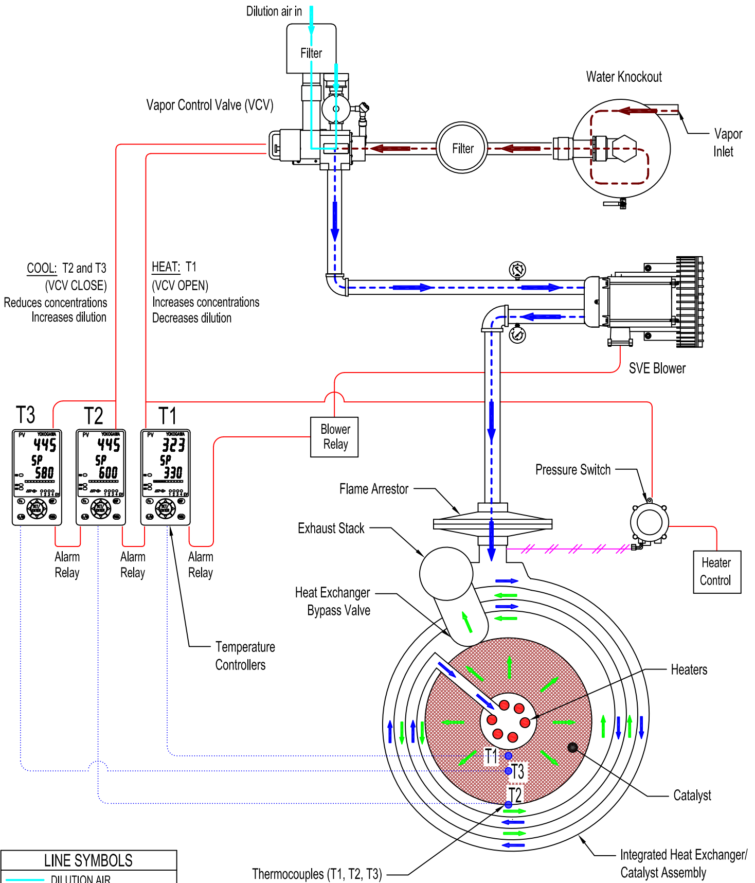
FIGURE 3: FALCO 600 FLOW AND CONTROL
