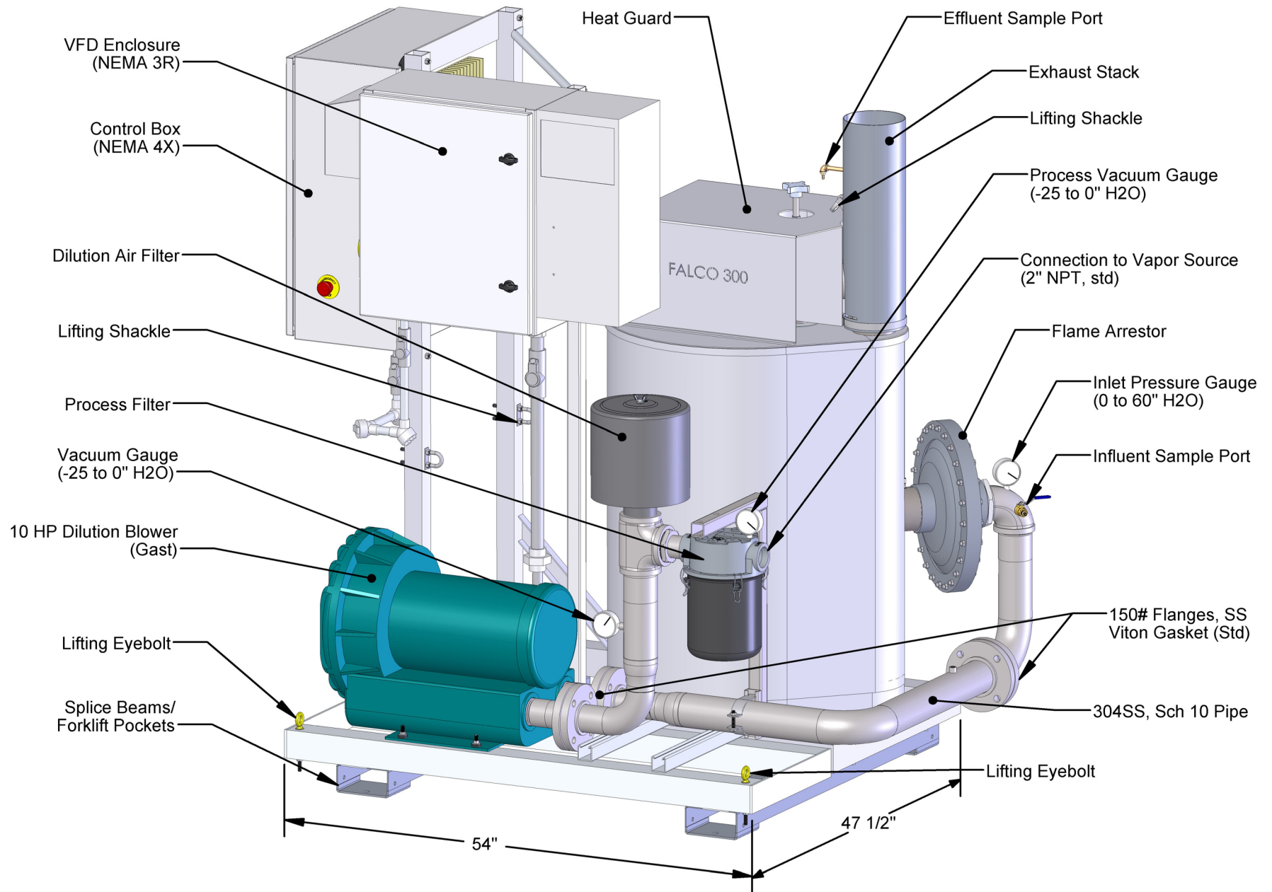
FIGURE 1B: FALCO 300 with VFD - Major Components
