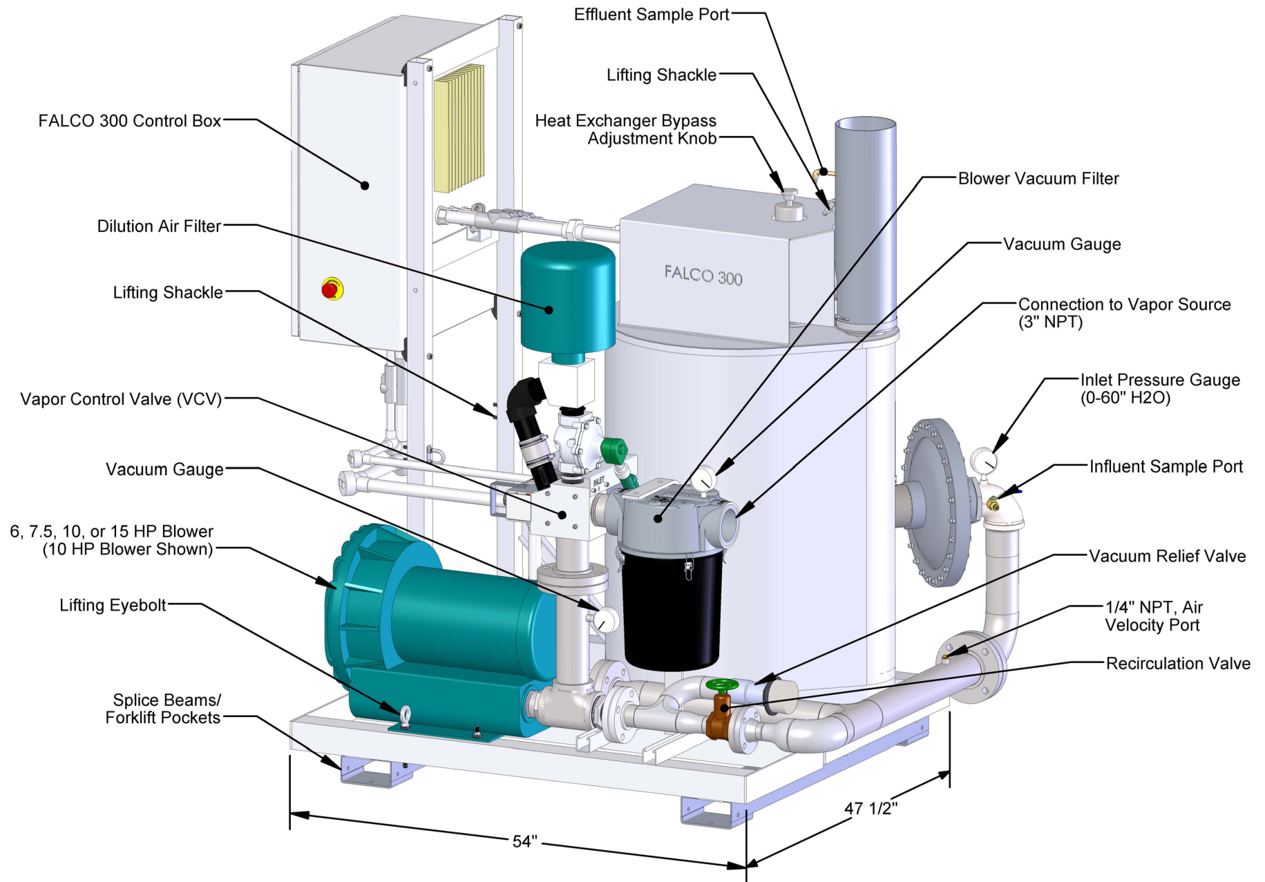
FIGURE 3: FALCO 300 with Regenerative Blower Package Major Components
