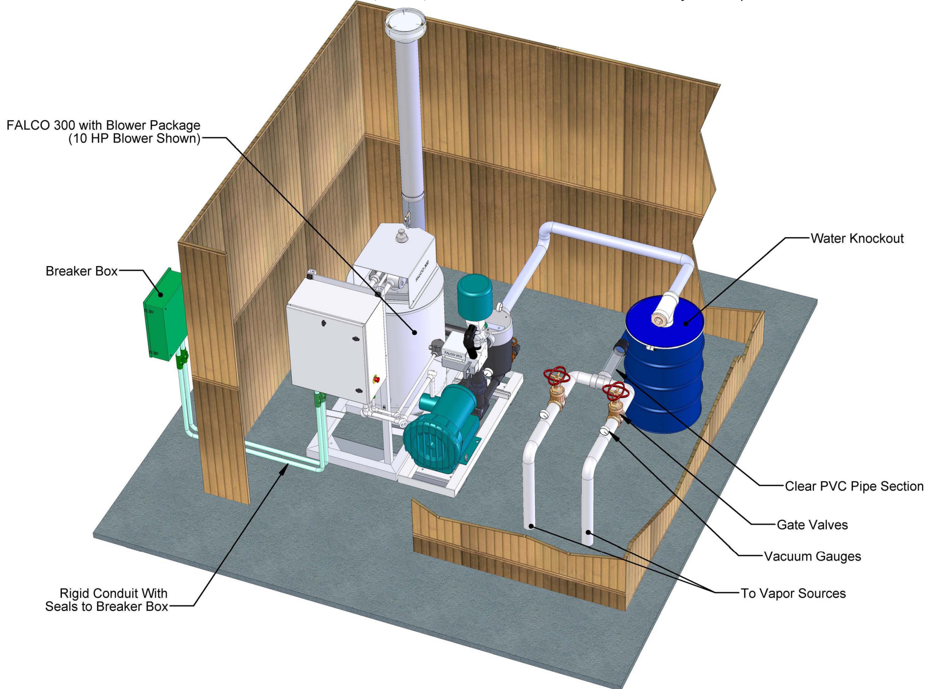
FIGURE 4: FALCO 300 Blower Package Site Installation
