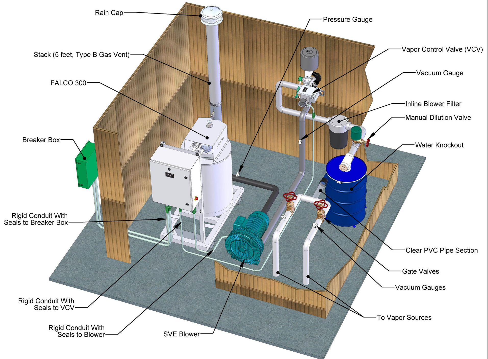
FIGURE 4: FALCO 300 Site Installation
