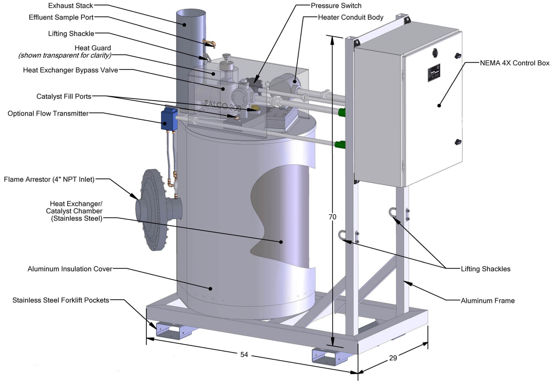
FIGURE 1: FALCO 300 - MAJOR COMPONENTS
