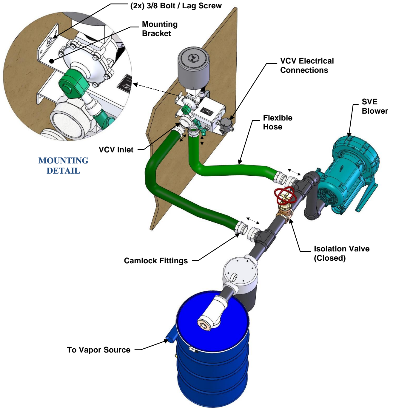
Figure 3 – TEMPORARY INSTALLATION
