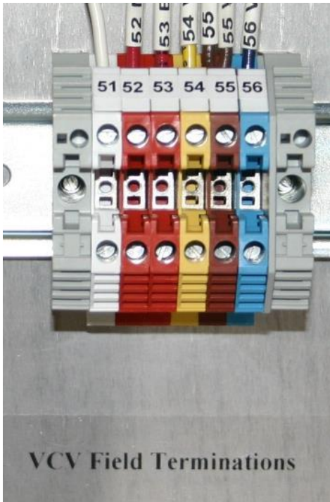
Figure 4 – FALCO Control Box Terminations
