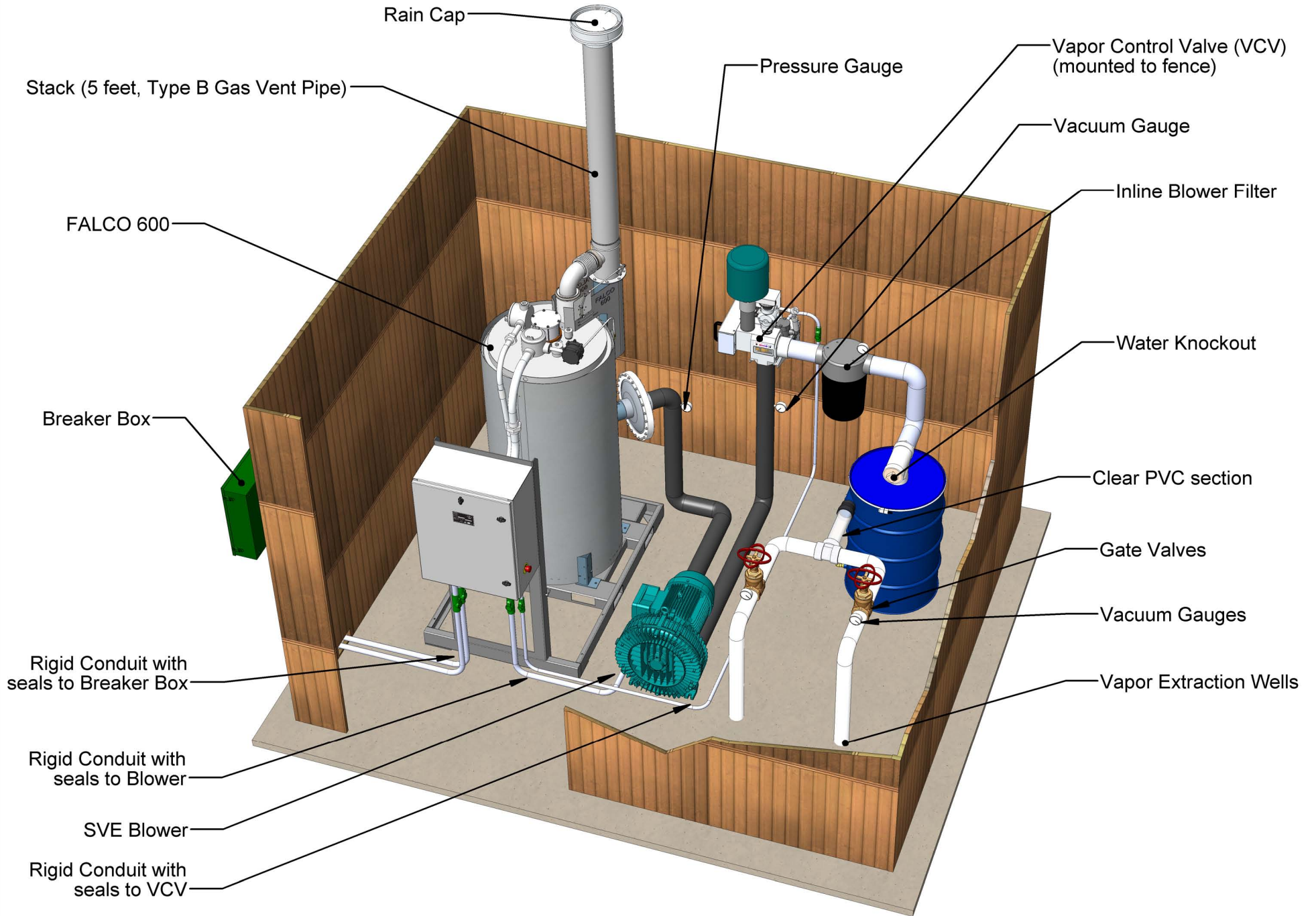
FIGURE 4: FALCO 600 Site Plan
