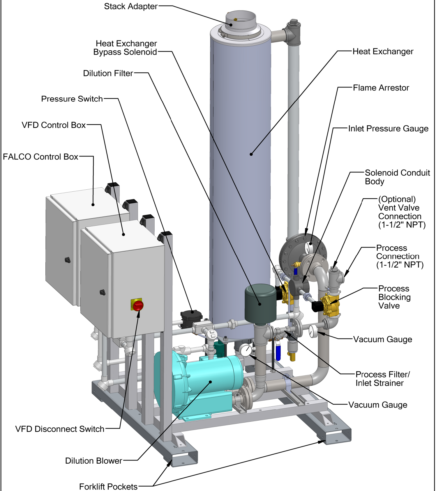
FIGURE 1B: FALCO 100 INDUSTRIAL, MAJOR COMPONENTS
