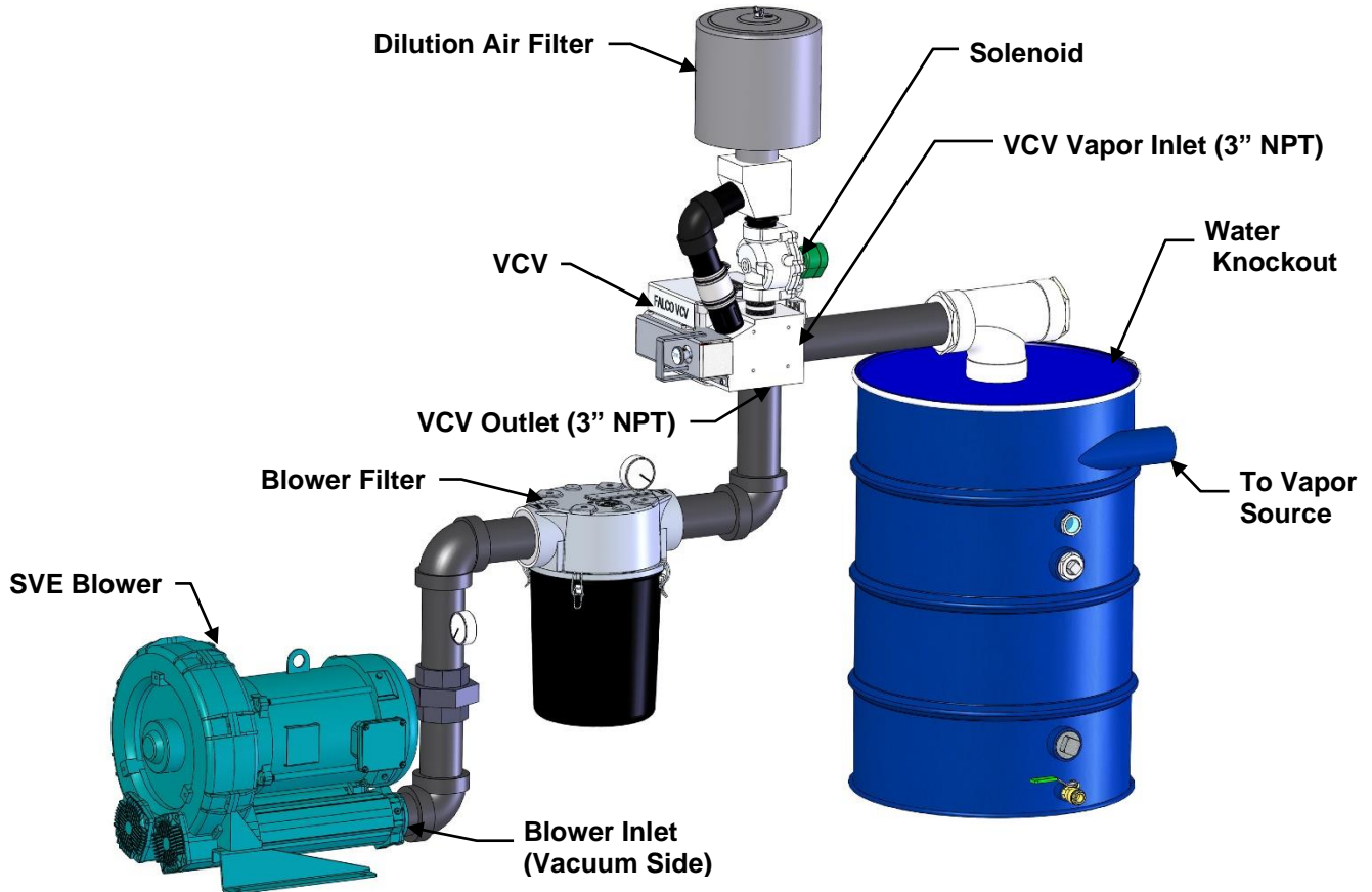
Figure 2 - ALTERNATIVE (LESS DESIRABLE) INSTALLATION
