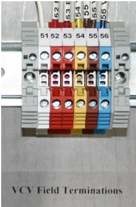
Figure 4 – FALCO Control Box Terminations
