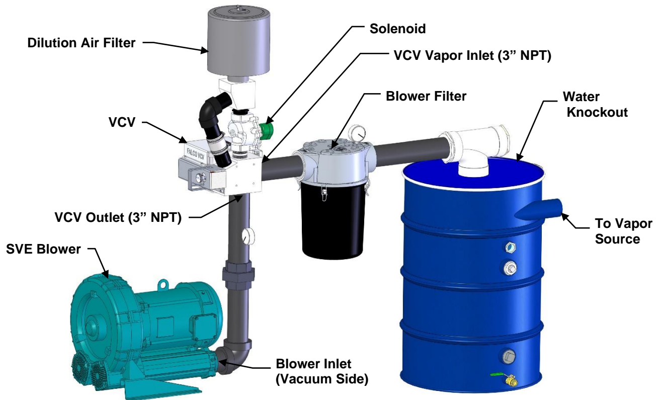
Figure 1 - PREFERRED INSTALLATION
