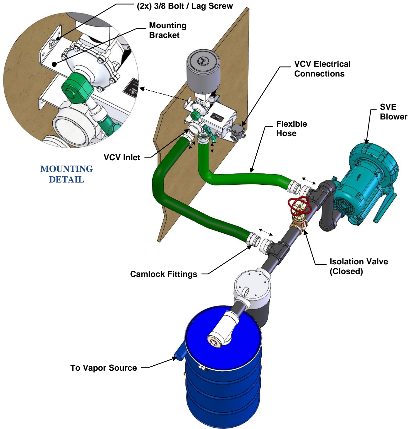
Figure 3 – TEMPORARY INSTALLATION
