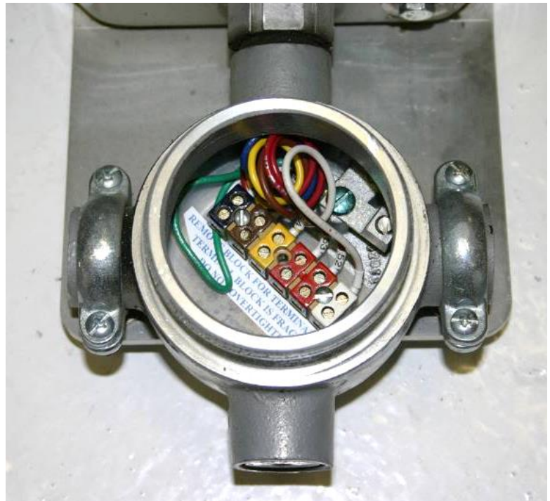
Figure 5 - VCV Conduit Body Terminations
