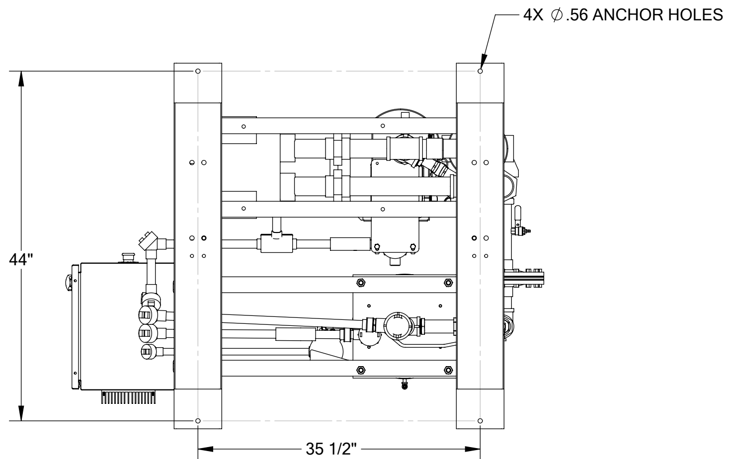
BOTTOM VIEW - ANCHOR HOLE LOCATIONS
