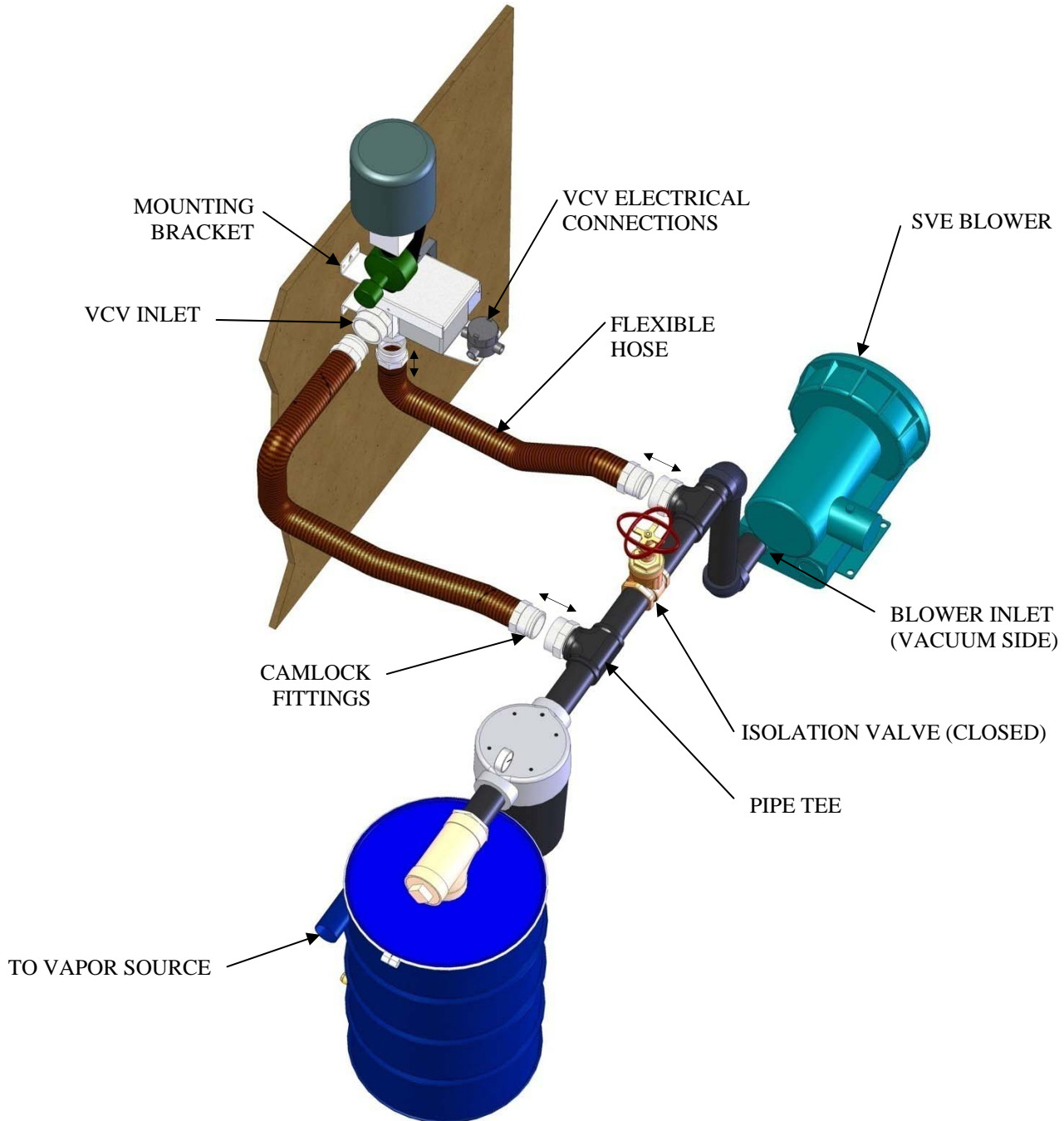
Figure 3 – TEMPORARY INSTALLATION
