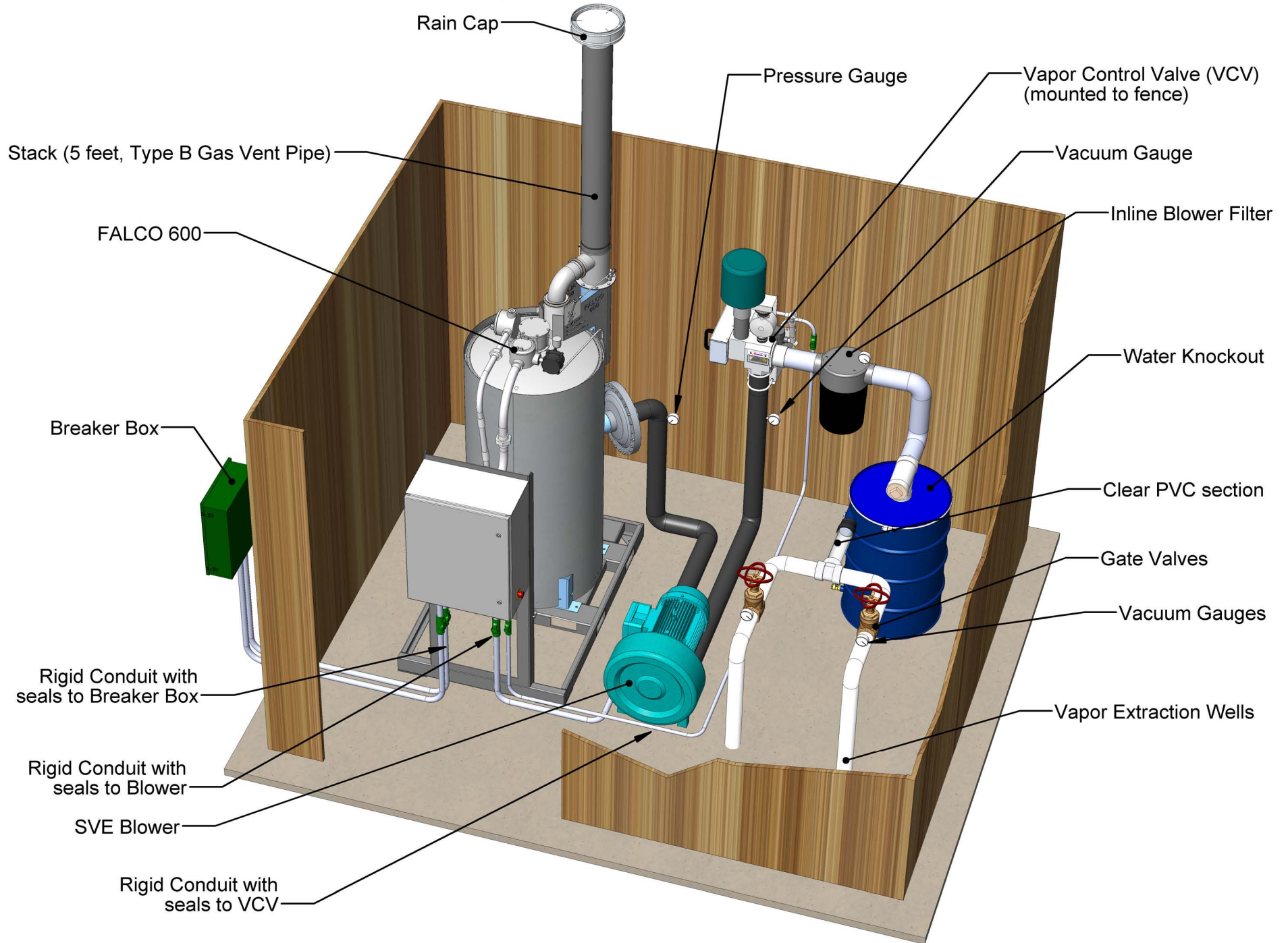
FIGURE 4: FALCO 600 Site Plan
