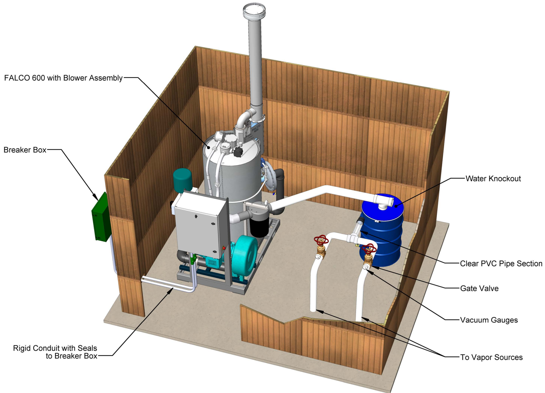
FIGURE 1: FALCO 600 with Regenerative Blower Assembly Site Installation
