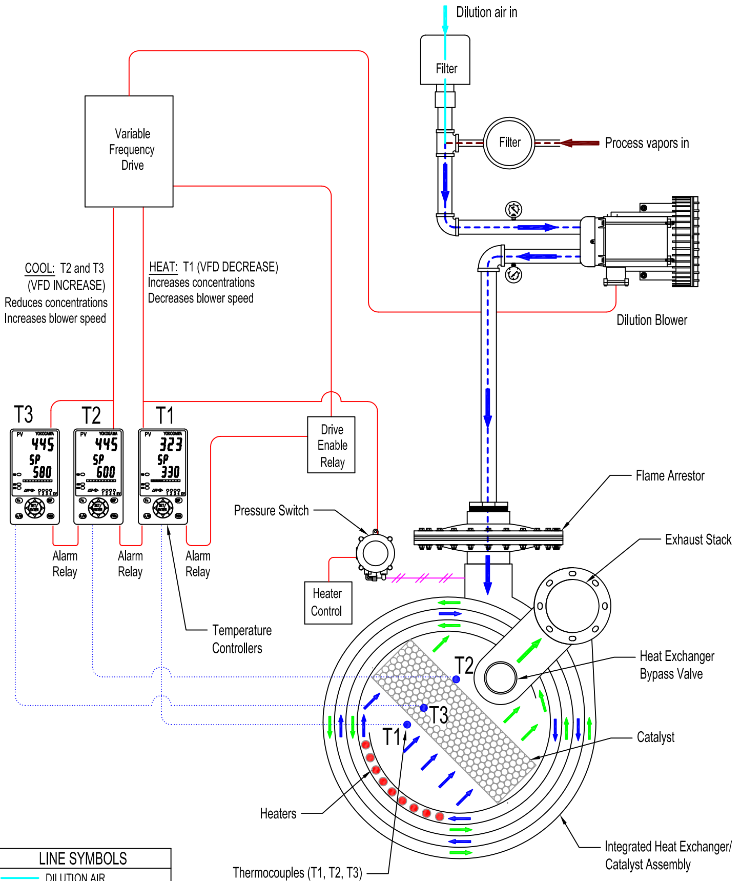
FIGURE 3B: FALCO 300 VFD FLOW AND CONTROL
