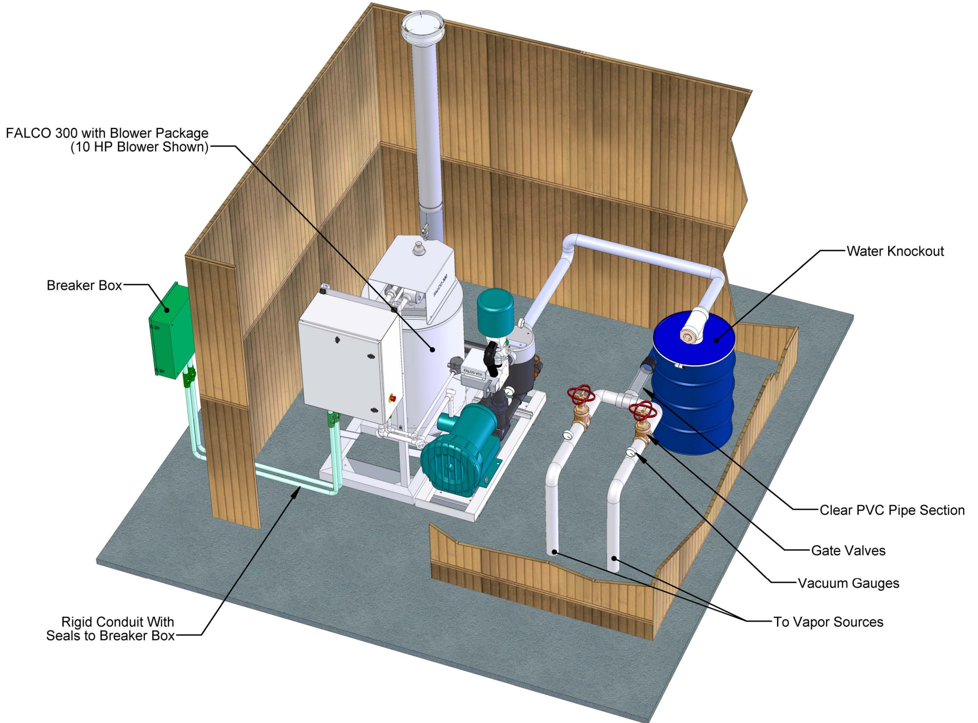
FIGURE 4: FALCO 300 Blower Package Site Installation
