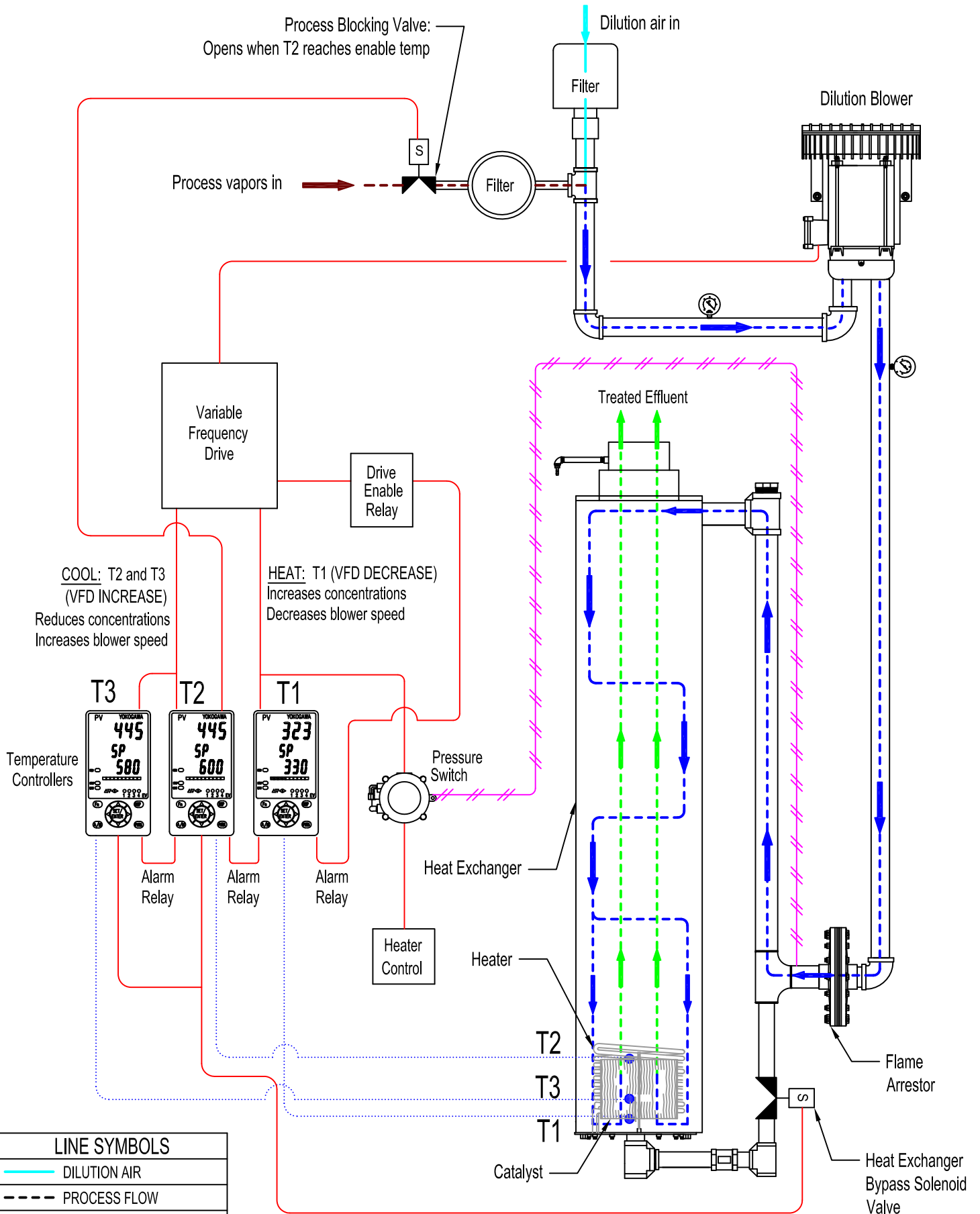
FIGURE 3B: FALCO 100 VFD FLOW AND CONTROL
