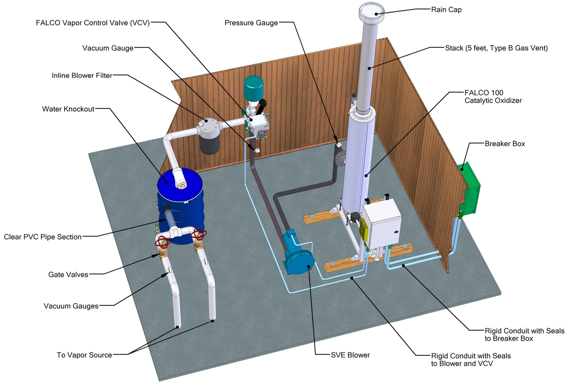
FIGURE 3: FALCO 100 Site Installation
