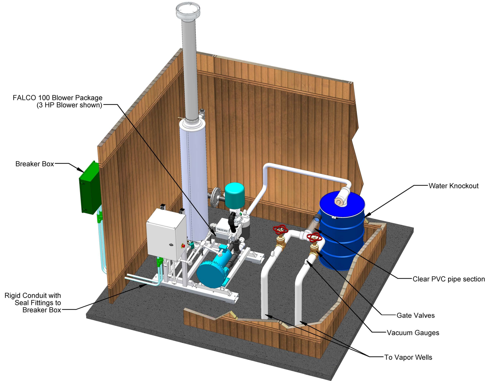
FIGURE 4: FALCO 100 BLOWER PACKAGE Site Installation
