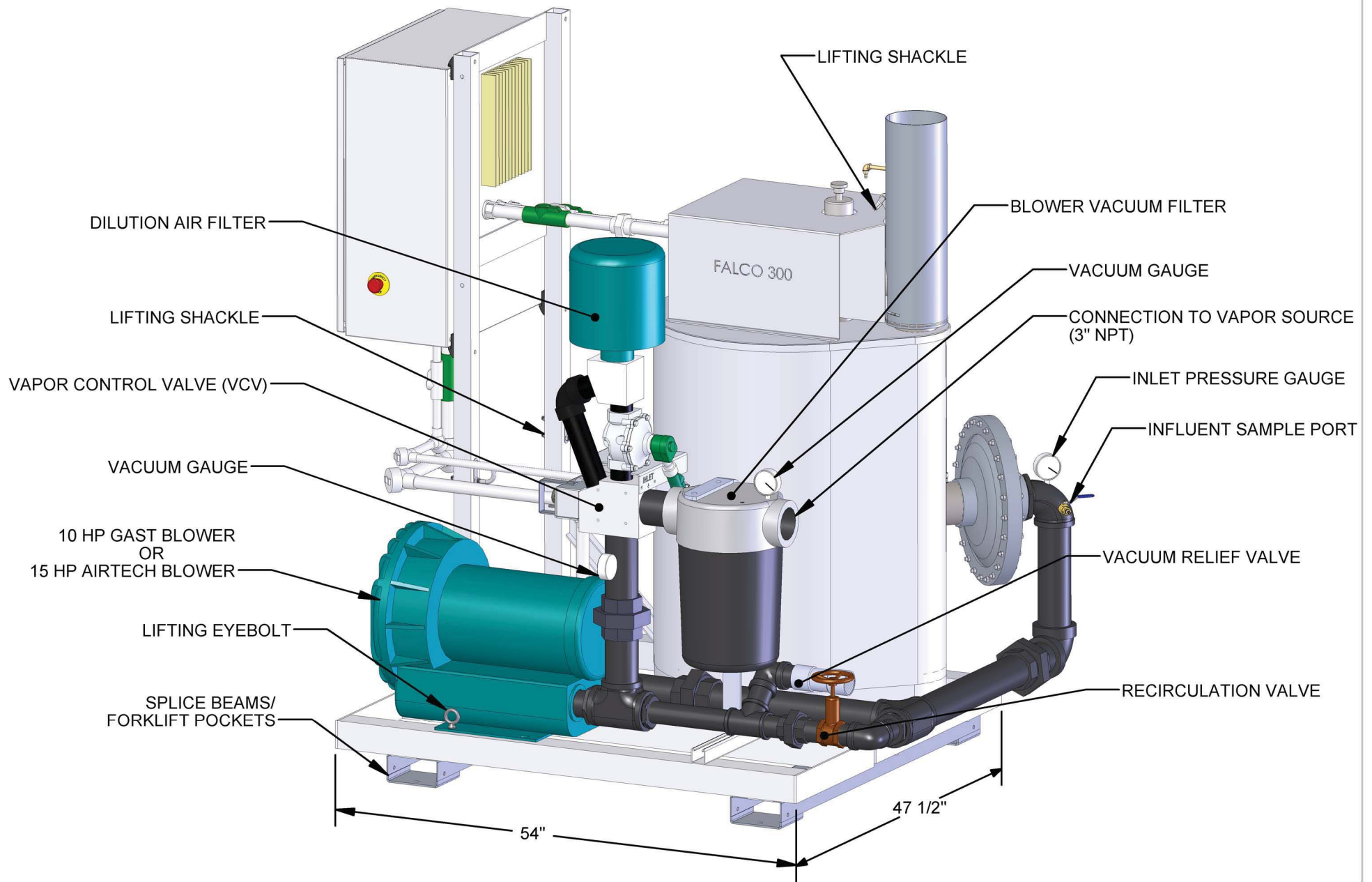
FALCO 300 with Regenerative Blower Package
