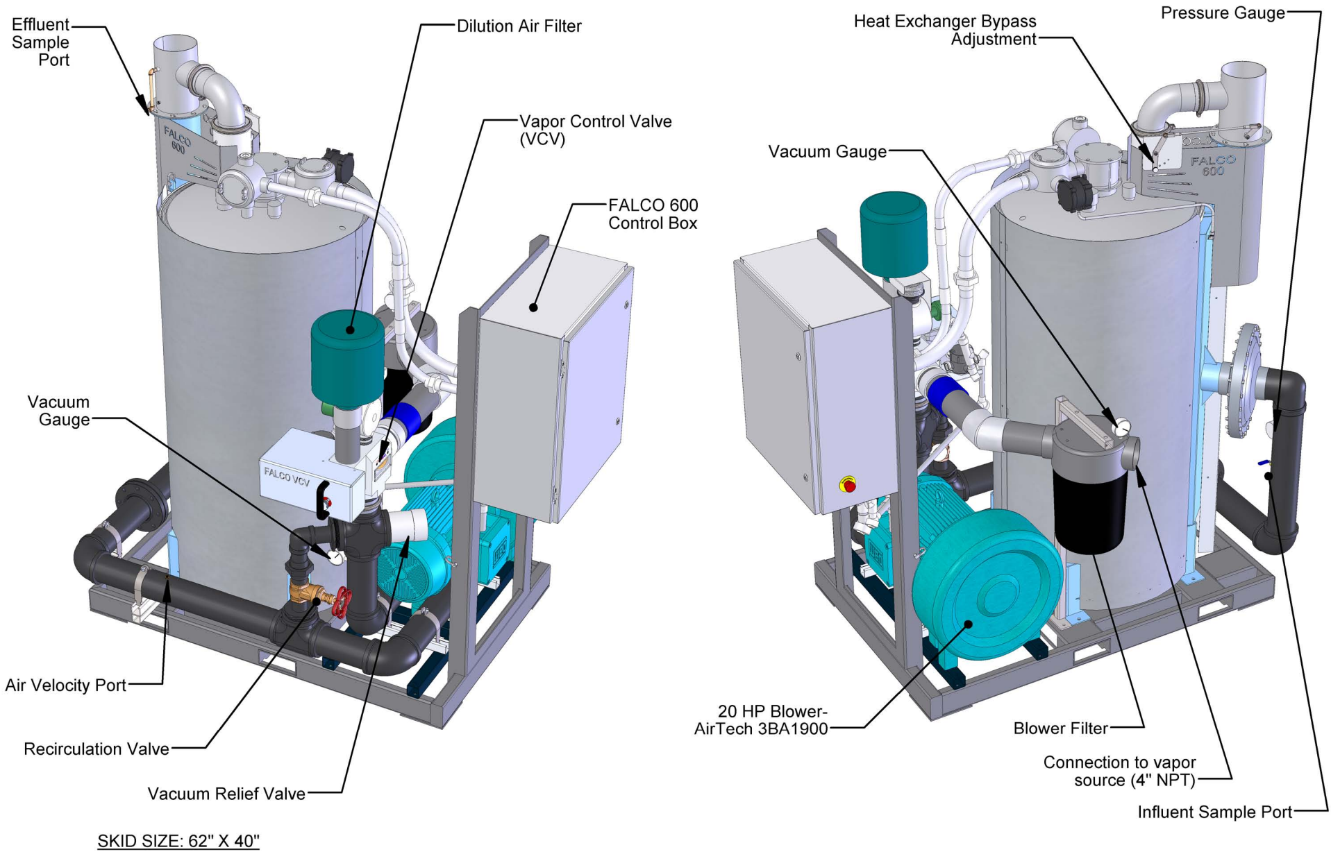
FALCO 600 with Regenerative Blower Assembly
