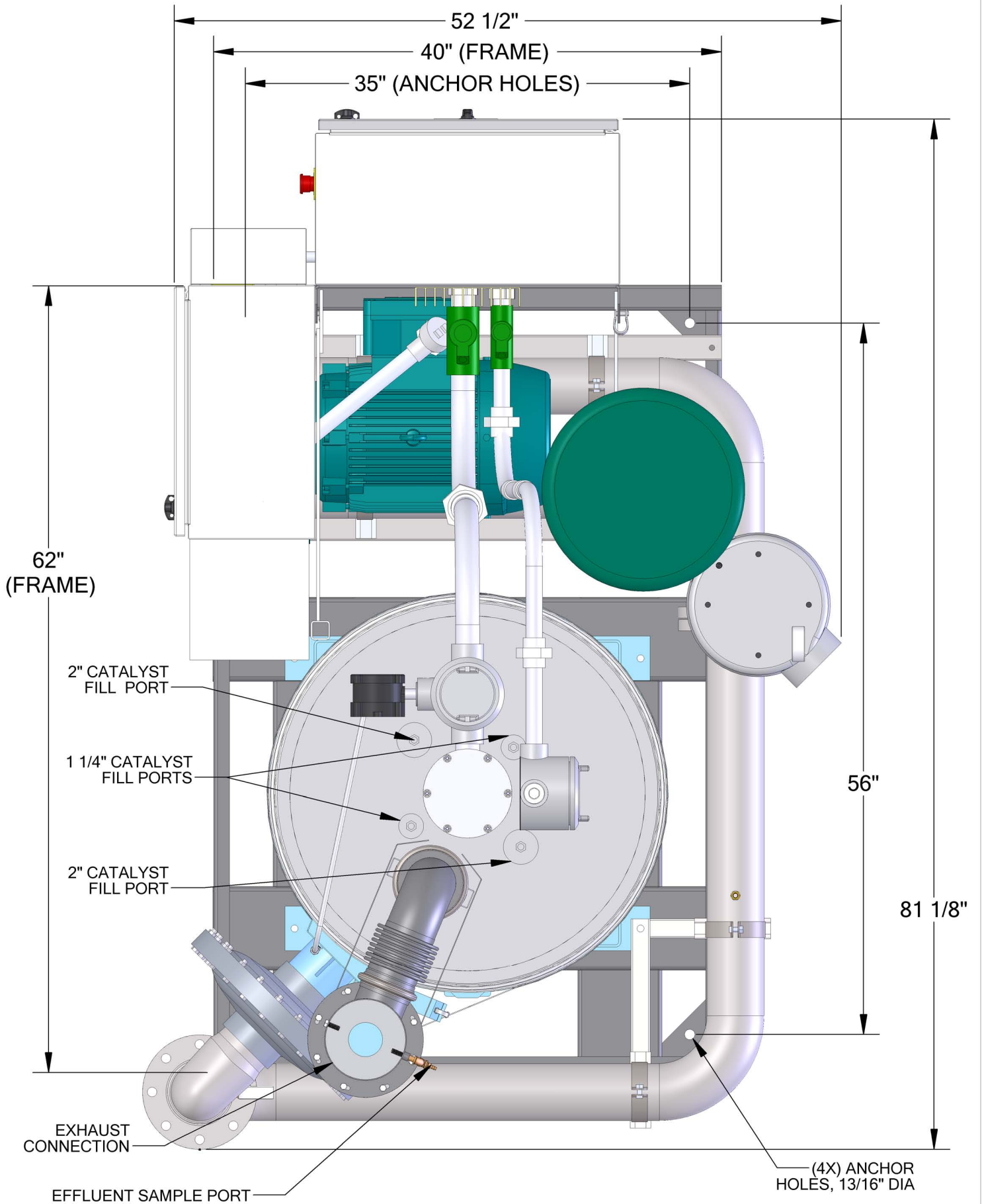
FIGURE 2B: FALCO 600 with VFD- TOP VIEW
