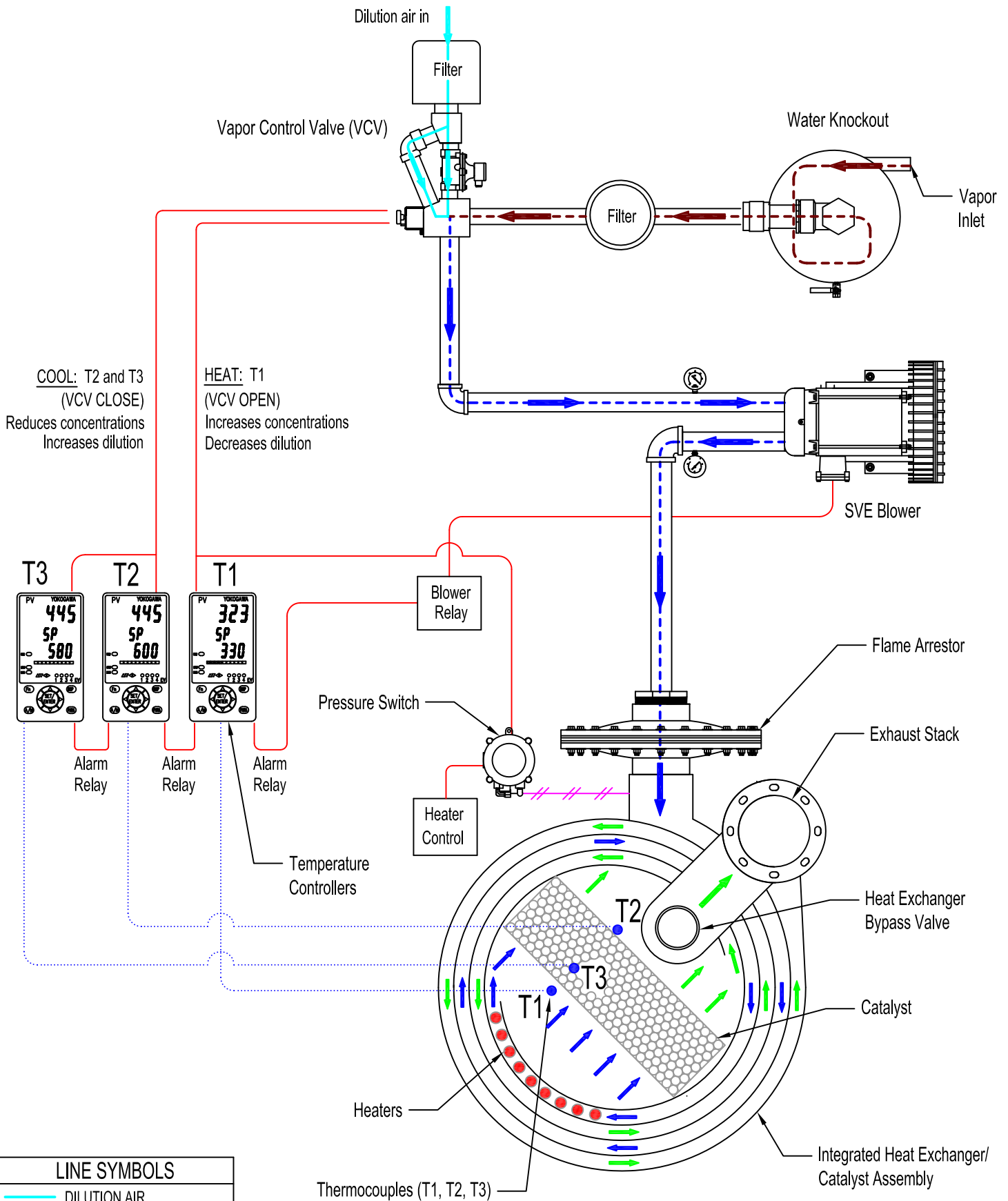
FIGURE 3: FALCO 300 FLOW AND CONTROL
