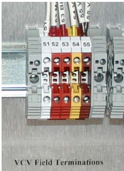
Figure 4 – FALCO Control Box Terminations
