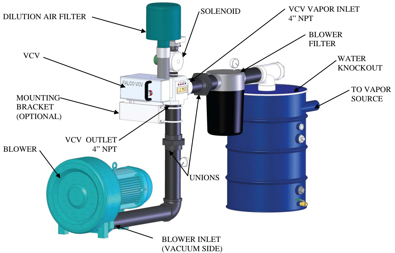
Figure 1 - PREFERRED INSTALLATION
