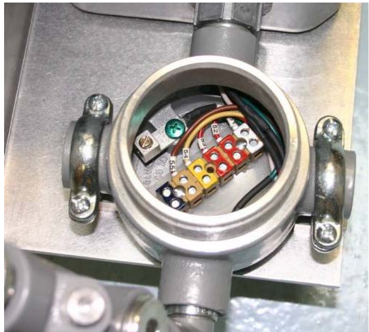
Figure 5 - VCV Conduit Body Terminations
